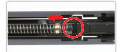
Push forward the recoil spring guide rod and compress the recoil spring.
